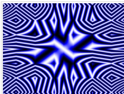
In modern notation, simple expressions can describe complex concepts. This image shows the graph of \cos(y \arccos \sin|x| + x \arcsin \cos|y|) .
